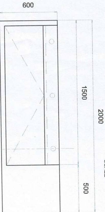
SECOND FLOOR-TAHANANG TEODORA ALONSO CONCRETE RAMP SINK PLAN SCALE 1:20
