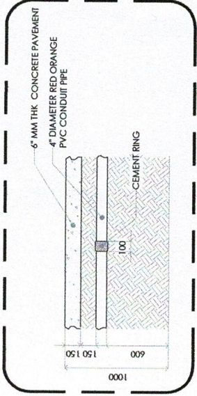
4 PIPE CONNECTION DETAILS E-01 SCALE: 1:50
